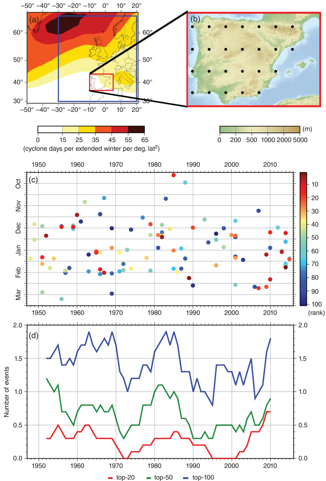
Figure 1. (a) Cyclone track density [cyclone days per extended winter season per deg. lat 2 ]; red box: geographical location of Iberian Peninsula; blue box: area for identification of cyclone tracks, (b) orography and NCEP grid points of investigated region, (c) time distribution of top-100 potential wind loss events for winters 1949–2015. Year corresponds to January, e.g. 1990: winter 1989/1990. Colours: rank of event (d) 10-year running mean of the number of events for each winter; red: top-20 potential wind losses; green: top-50, blue: top-100 wind loss events; e.g. 1953: running mean of 1949–1958. Average number of events per winter: top-100 potential wind losses: 1.5; top-50: 0.75; top-20: 0.3.
