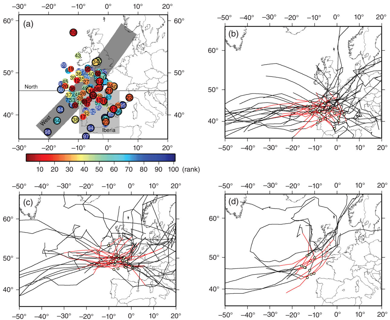
Figure 2. (a) Position of minimum pressure of identified cyclones responsible for potential wind losses over the Iberian Peninsula at the event day. Colours/numbers: rank of event; black circle: cyclones associated with Hybrid type. Identification of regions of the different groups: Iberia (light grey shaded region): cyclones crossing this area during the event day; North: cyclones crossing from west to east in a zonal path within this region during the event day; West (dark grey shaded region): cyclones crossing from southwest to northeast along the dark grey shaded region. (b) Cyclone tracks of group Iberia (31 events). (c) Cyclone tracks within North (28 events). (d) Cyclone tracks for West group (11 events). (b)–(d) red: cyclone track during the event day; circles: corresponding to (a).
