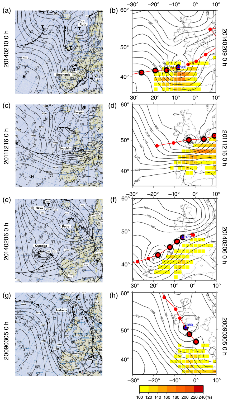
Figure 3. Case study for (a, b) group Iberia , (c, d) group North , (e, f) group West , (g, h) group Hybrid . Left panels: surface weather charts adapted with courtesy of Berliner Wetterkarte e.V.; right panels: windstorm footprints and responsible cyclone tracks; black circle: time frames corresponding to event day, blue triangle: pressure minimum at event day [for (d) outside shown area]; colours: exceedance of v_{98} in (%); date: yyyyymmdd time in UTC.
