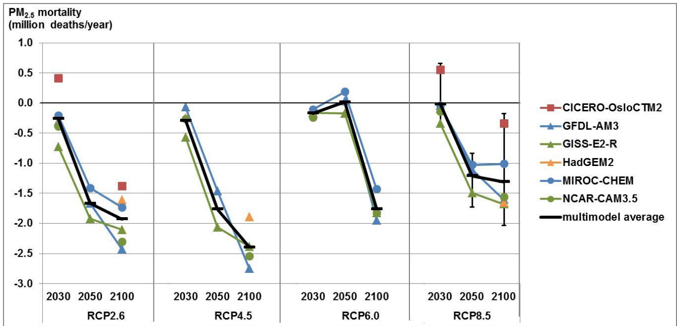
Figure 4: Estimates of future premature mortality (IHD+STROKE+COPD+LC) for PM_{2.5} calculated as a sum of species, for all RCP scenarios in 2030, 2050 and 2100, showing global mortality for six models and the multi-model average (million deaths/year), for future air pollutant concentrations relative to 2000 concentrations. Uncertainty shown for the RCP8.5 multi-model average is the 95% CI including uncertainty in RR and across models.
