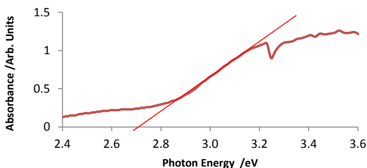
Figure 7: Diffuse reflectance spectrum of (H_{1.33}tren)[In_{2.67}Sb_{1.33}S_8] \cdot tren
