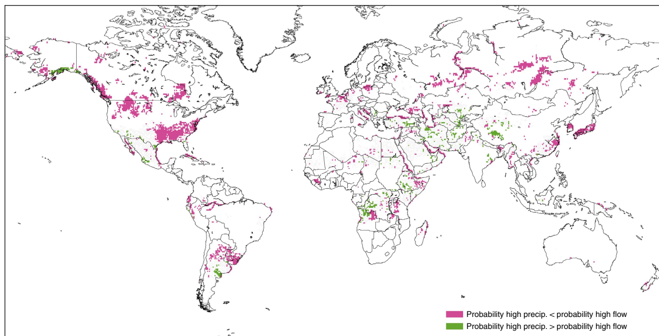
Figure 3 | Comparison of historical probabilities based on precipitation and river flow. Regions where the difference in probability of abnormally high precipitation compared to probability of high river flow, in the month of February during an El Niño, is greater than 10% (based on the ensemble mean). Pink shading indicates that the probability of high precipitation is smaller than the probability of high river flow, while green shading indicates that probabilities are larger for precipitation.
