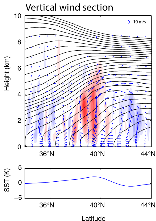
FIG. 8. (top) Meridional cross section of the difference between CNTL and SMTH in wind (arrows) and vertical wind (color shading) averaged between longitudes 65° and 45°W over the third day of the simulation. Potential temperature (every 2 K) is overlaid in black contours. (bottom) CNTL minus SMTH SST (K) averaged over the same range of longitudes as fields in (top).
