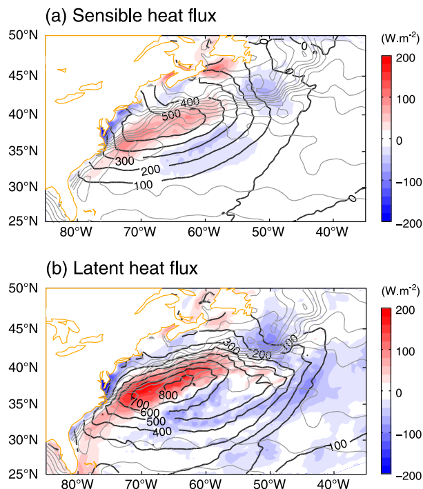
FIG. 9. Surface turbulent in (a) sensible and (b) latent heat fluxes ( W m^{-2} ) in CNTL (black contours) and their difference with SMTH (color shading) over the third day of the case study. The gray contours represent CNTL SST (every 2 K).
