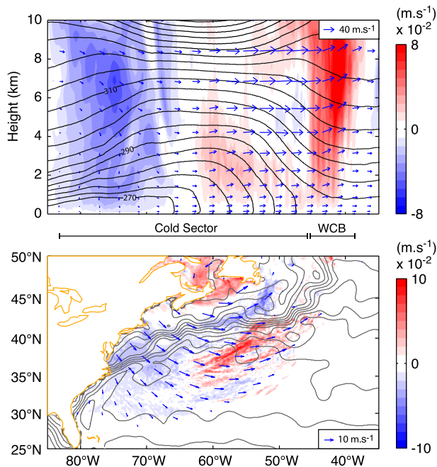
FIG. 4. (top) Zonal cross section of wind in CNTL (arrows) and vertical wind only (colors) averaged between 36° and 42°N. Potential temperature (every 4 K) is overlaid in black lines. (bottom) Vertical wind at 700 hPa in the cold sector in CNTL. The cold-sector contribution was selected by applying the cold-sector mask and WCB's contribution is not shown. Arrows stand for 10-m wind vectors. The gray contours represent CNTL SST (every 2 K). All the diagnostics are 24-h averaged over the third day of the simulation.
