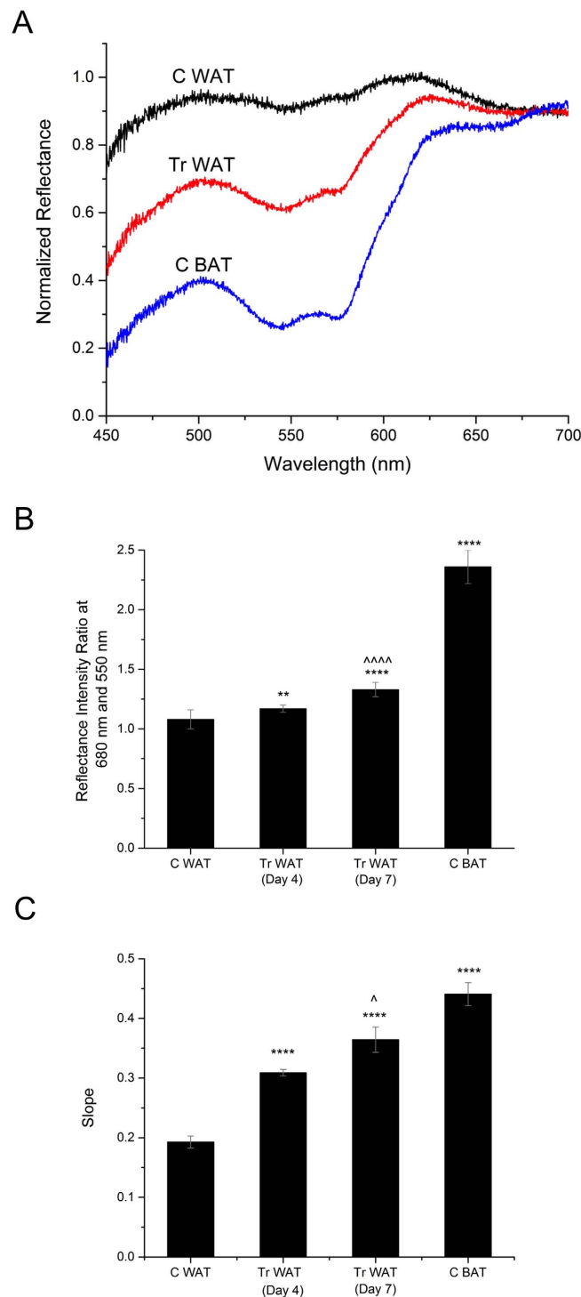
Figure 2. Representative normalized DRS spectra from adipose tissues (A). Reflectance intensity ratio at 680 and 550 nm of adipose tissues (B) and slope value in the 570–630 nm range for adipose tissues (C). ** p < 0.01 and **** p < 0.0001 denote significance when compared to C WAT; ^ p < 0.05 and ^^^^ p < 0.0001 denotes significance in Tr WAT (Day 7) when compared to Tr WAT (Day 4) ( n = 4-8 ).
