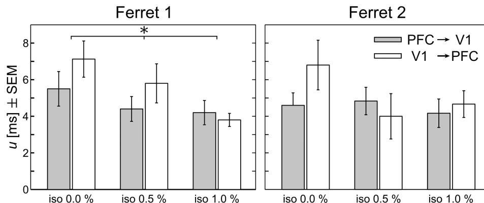
Fig 6. Optimized information transfer delays u for both directions of interaction and three levels of isoflurane, by animal. Bars denote averages over recordings per condition; error bars indicate the standard error of the mean (SEM). There was a significant main effect of isoflurane level for ferret 1 ( p < 0.05 ).
