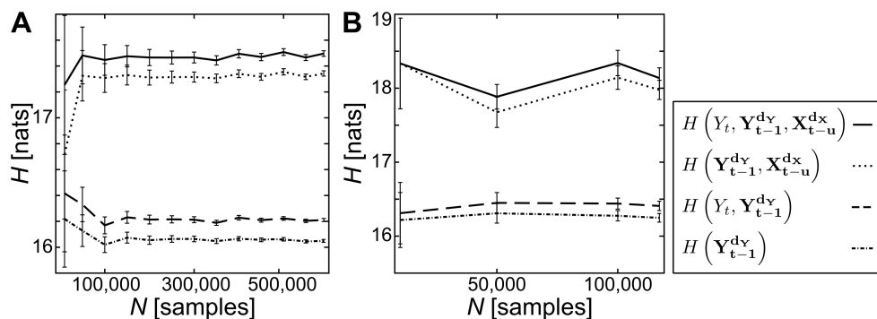
Fig 3. Examples for estimates of entropy ( H ) terms for transfer entropy calculation (Eq 12) by number of data points N , using the Nemenman-Shafee-Bialek-estimator (NSB). (A) entropies for ferret 1, V1, iso 0.5%: estimates are stable for N \geq 100,000 ; (B) entropies for ferret 2, PFC, iso 0.0%: an insufficient number of data points does not allow for verification of the estimate's robustness (recording was excluded from further analysis). Variables labeled X reflect data from the source variable, Y from the target variable. t is an integer time index, and bold typeface indicates the state of a system (see Methods).
