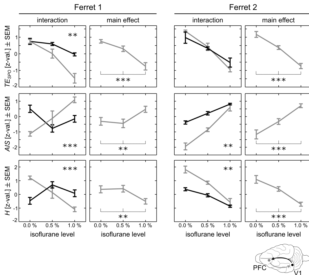
Fig 1. pANOVA results for nearest-neighbor based estimates of transfer entropy ( TE_{SPO} ), active information storage (AIS), and entropy ( H ). Left columns show interactions isoflurane level \times direction and isoflurane level \times recording site for both animals; right columns show main effects isoflurane level . Grey lines in interaction plots indicate TE_{SPO} from prefrontal cortex (PFC) to primary visual areas (V1), or H and AIS in PFC; black lines indicate TE_{SPO} from V1 to PFC, or H and AIS in V1. Error bars indicate the standard error of the mean (SEM); stars indicate significant interactions or main effects (* p < 0.05 ; ** p < 0.01 ; *** p < 0.001 ). Axis units for all information theoretic measures based on continuous variables are z-normalized values across conditions.
