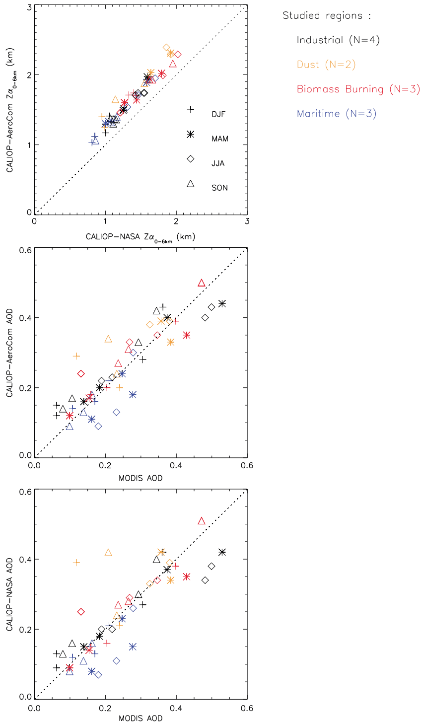
Figure 3. The 2007 Z\alpha_{0-6 km} mean seasonal extinction height over the 12 selected regions: (top) AeroCom (this study) versus NASA [Winker et al., 2013] 2007 CALIOP gridded products. The 2007 mean seasonal AOD, over the 12 selected regions as derived from the (middle) AeroCom (this study) and (bottom) NASA [Winker et al., 2013] CALIOP gridded products, compared to 2007 MODIS measurements.
