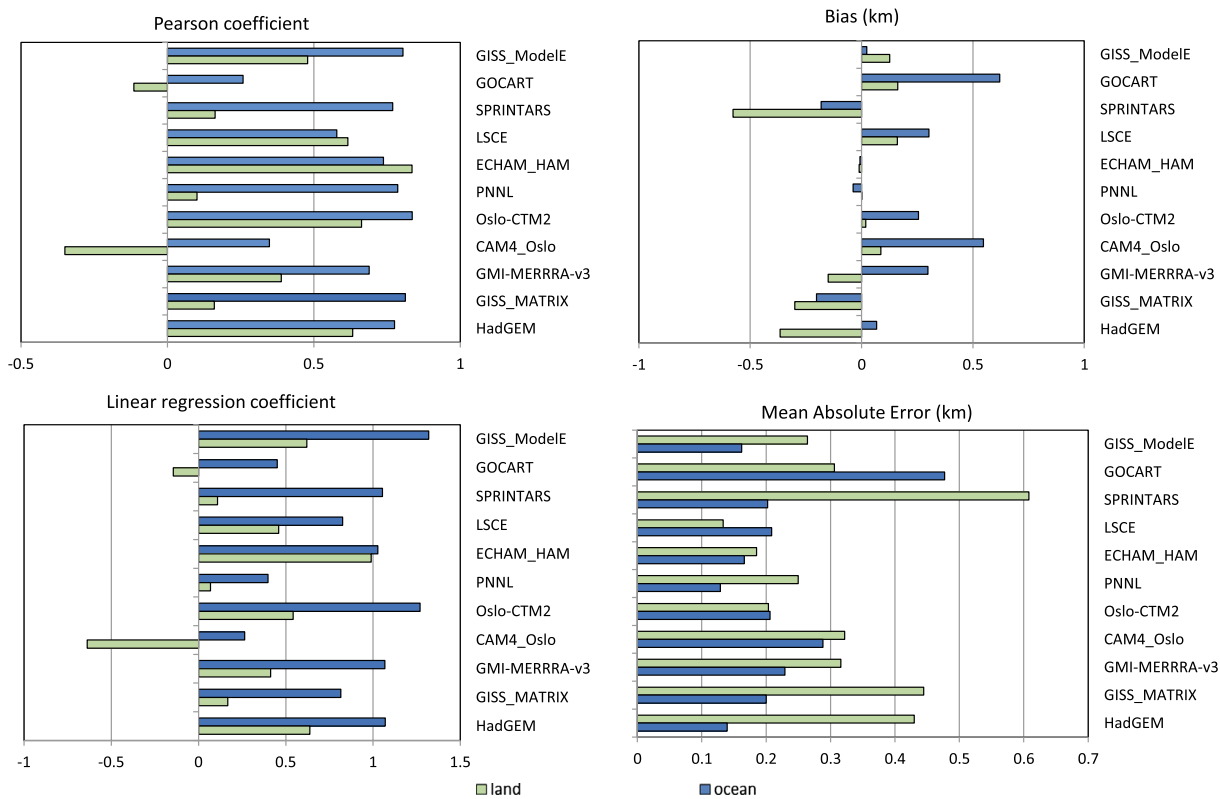
Figure 10. Comparison of AeroCom II (2006) models performance in reproducing CALIOP (2007–2009) mean annual Z_{\alpha 0-6 \text{ km}} aerosol extinction height over land (green) and ocean (blue): (top left) Pearson coefficient (threshold value for p = 0.05 is 0.532); (bottom left) linear regression coefficient, and (bottom right) mean absolute error (km) and (top right) bias (km).
