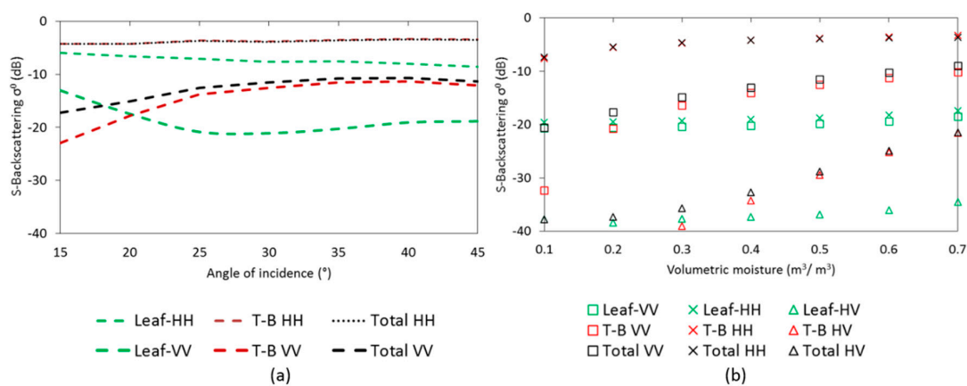
Figure A1. S-band backscatter vs. canopy parts (a) at 0.5 volumetric moisture ( m^3/m^3 ) across incidence angles and (b) at varying volumetric moisture ( m^3/m^3 ) at 30^\circ radar range where T- and B- represents trunk and branches respectively.
