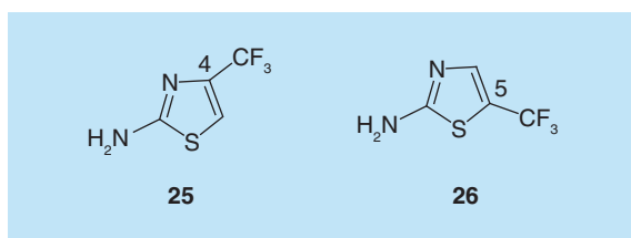
Figure 4. 2-Amino-[4'- and 5'-(trifluoromethyl)]thiazoles.
