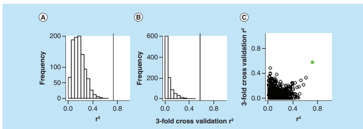
Figure 7. Validation of the regression model. (A) Histogram of r^2 values from 1000 iterations of randomly permuted influenza A activity values (true data r^2 shown as solid vertical line at 0.72). (B) Histogram of threefold cross-validation r^2 values from 1000 iterations of randomly permuted influenza A activity values (true data r^2 shown as solid vertical line at 0.58). (C) Plot of r^2 and threefold cross-validation r^2 values from 1000 iterations of randomly permuted influenza A activity values as black circles, with the statistical measures from the true data displayed as a solid green circle.
