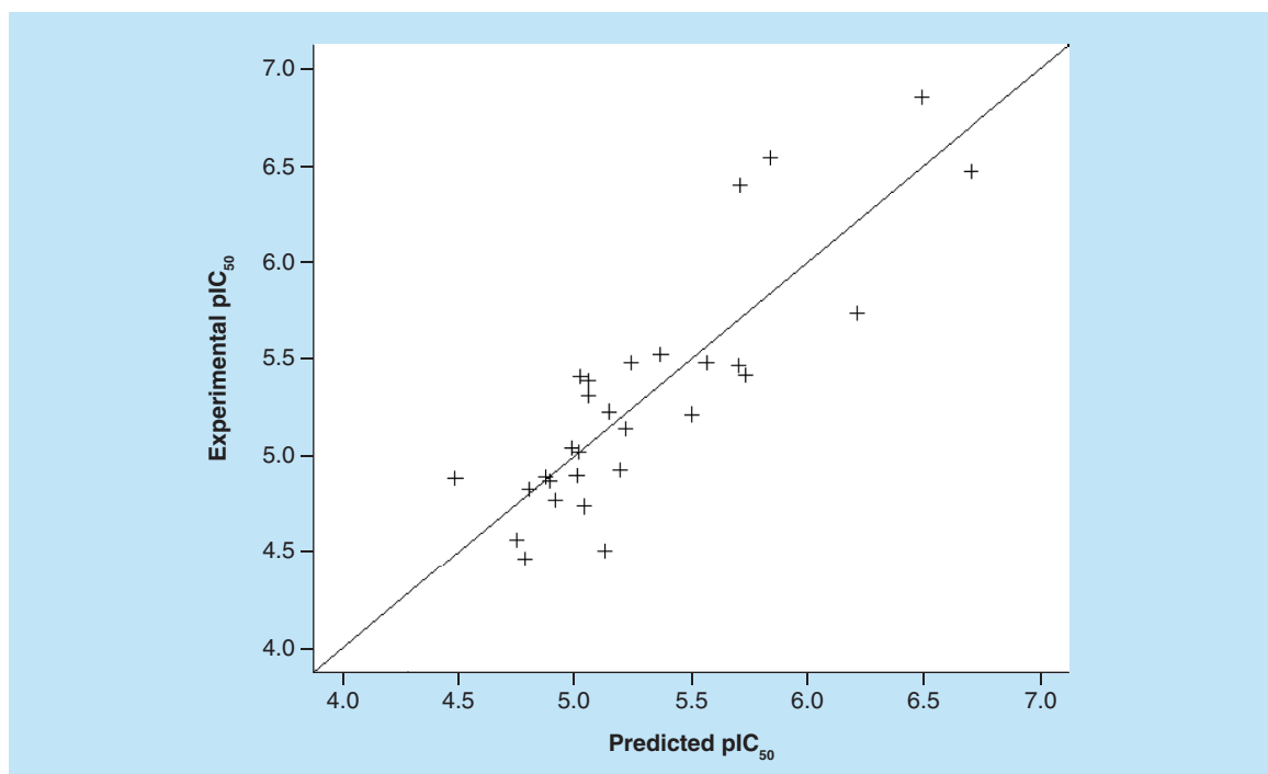
Figure 6. Genetic algorithm-multiple linear regression regression model for influenza A (PR8) Madin–Darby canine kidney cells. Further validation of the statistical significance of this model was obtained through randomization of the activity data and calculation of the r^2 and threefold cross-validation r^2 on the permuted data. This process was repeated 1000-times and the results are plotted in. As can be seen from the histograms of the permuted models for r^2 and cross-validated r^2 (Figures 7A & B), the randomized data do not produce models that perform anywhere near as well as with the true data (indicated by the single vertical lines). Figure 7C displays the model built on the experimental data as a filled green circle, and yet again, none of the permuted models perform as well as the genuine dataset. This series of tests indicates the high significance of the quantitative structure–property relationship model derived from the measured data.
