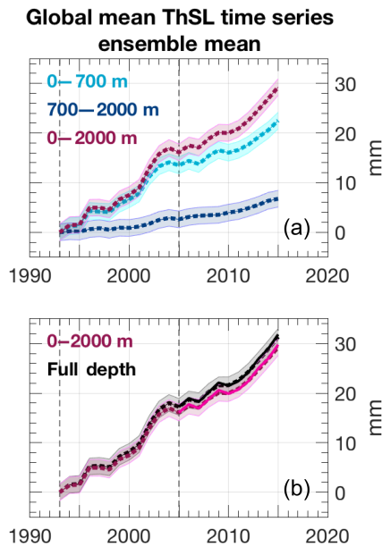
Figure 6. Ensemble mean time series for global mean thermosteric sea level anomaly, for three depth integrations (a) and for 0–2000 m and full depth (b). In the bottom panel, dashed lines are for the 1993–2015 period whereas solid lines are for 2005–2015. Error bars represent the ensemble spread (standard deviation). Units are millimeters.
