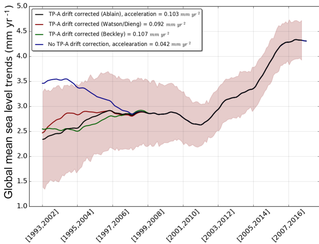
Figure 3. Ensemble mean GMSL trends calculated over 10-year moving windows. On the black, red and green curves, the TOPEX-A drift correction is applied respectively based on Ablain et al. (2017b), Watson et al. (2015) and Dieng et al. (2017), and Beckley et al. (2017). Uncorrected GMSL trends are shown by the blue curve. The shaded area represents trend uncertainty over 10-year periods (90 % confidence interval).
