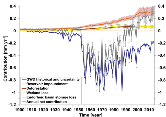
Figure 11. Time series of the estimated annual contribution of terrestrial water storage change to global sea level over the period 1900–2014 (rates in millimeters per year of SLE) (modified from Wada et al., 2016).
