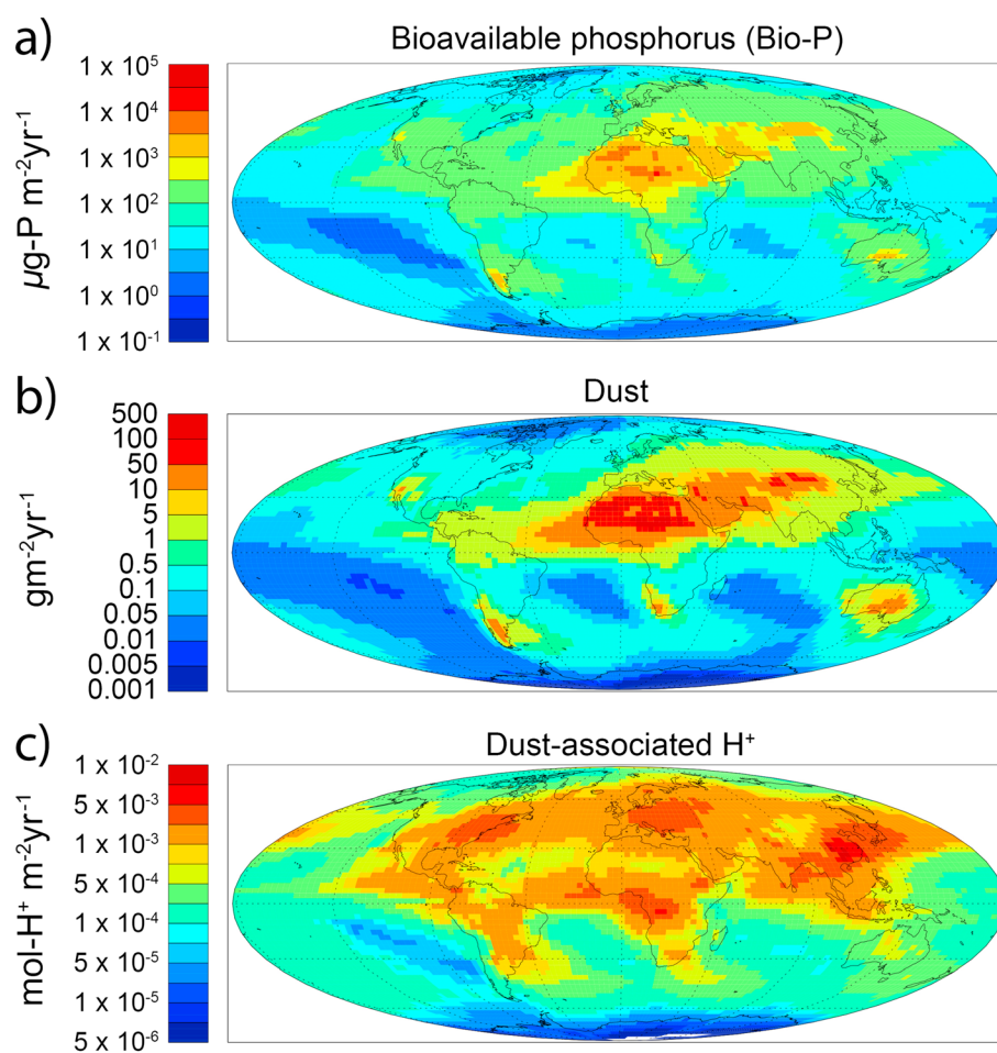
Figure 2. Annual deposition rate of (a) bioavailable phosphorus in \mu\text{g-P/m}^2/\text{year} , (b) dust in \text{g/m}^2/\text{year} , and (c) dust-associated \text{H}^+ ions in \text{mol-H}^+/\text{m}^2/\text{year} .
