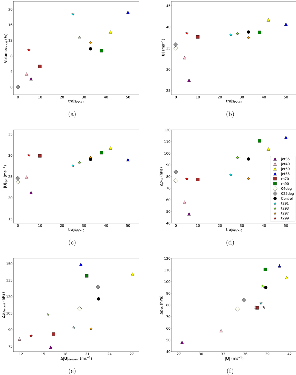
Figure 12. Scatterplots showing, for all the sensitivity experiments, (a) \text{volume}_{PV < 0} against \text{trajSPV} < 0 , (b) |\mathbf{U}| against \text{trajSPV} < 0 , (c) |\mathbf{U}|_{\text{sys}} against \text{trajSPV} < 0 , (d) \Delta p_{5h} against \text{trajSPV} < 0 , (e) \Delta p_{\text{descent}} against \Delta |\mathbf{U}|_{\text{descent}} and (f) \Delta p_{5h} against |\mathbf{U}| . \text{trajSPV} < 0 is the maximum number of trajectories of the 100 selected with negative PV at any instant within 15 h from the time when the trajectories are selected (i.e. identification time), and \text{volume}_{PV < 0} indicates the maximum percentage of grid points with negative PV, evaluated in the same time window as \text{trajSPV} < 0 , in a volume centred on the location of the median of trajectories and extending for 20 grid points in latitude, 40 grid points in longitude and three vertical pressure levels (note that the symbols for the reduced resolution simulations overlie at point (0,0) in panel a). |\mathbf{U}| is the maximum Earth-relative speed, |\mathbf{U}|_{\text{sys}} is the system-relative speed at the time when |\mathbf{U}| is reached, and \Delta p_{5h} is the maximum 5 h pressure increase in a period ending by identification time. \Delta p_{\text{descent}} and \Delta |\mathbf{U}|_{\text{descent}} indicate, respectively, total pressure increase and speed increment during the whole SJ descent, whose end is taken at identification time and whose start has to be not more than 12 h before. All these kinematic quantities refer to the median of trajectories.
