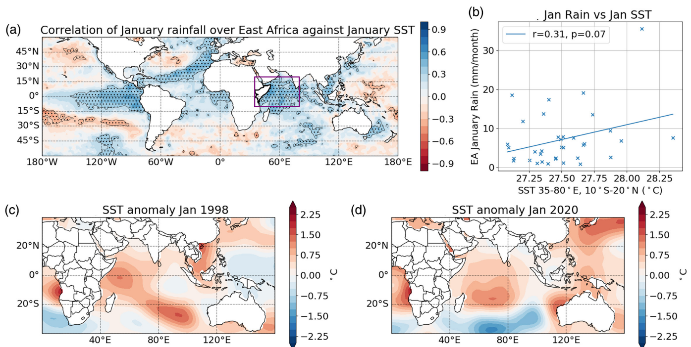
Figure 6. Correlation of January rainfall over Eastern Africa (region in black, TAMSATv3) against HadISST SST over 1985–2019; stippling indicates where the correlation is significant at the 10% level (a). (b) shows the scatter plot of mean January rainfall over Eastern Africa (black region, TAMSATv3) against mean January SST (HadISST) over the purple box shown in (a) for 1985–2019. (c, d) show the SST anomaly in January 1998 and January 2020. For (c and d) SST anomalies are relative to 1981–2010 and are taken from NOAA Extended SST V4 (SST); https://www.esrl.noaa.gov/psd/cgi-bin/data/composites/printpage.pl .
