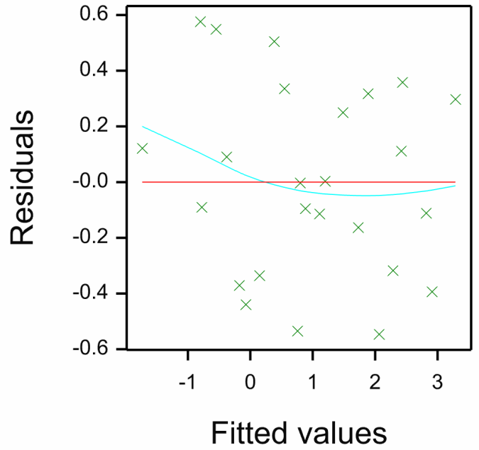
Fitted-value plot
