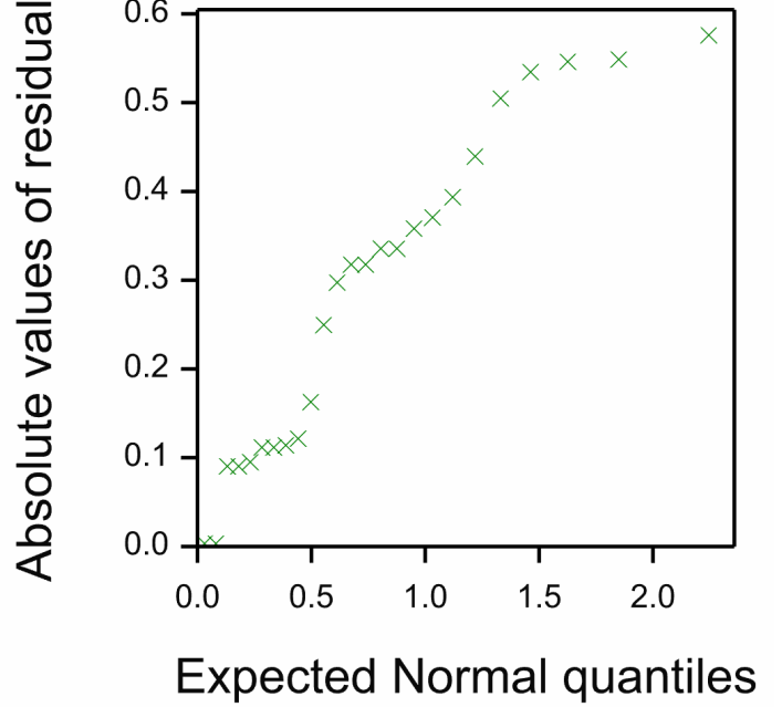
Half-Normal plot
