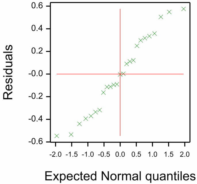
Normal plot
