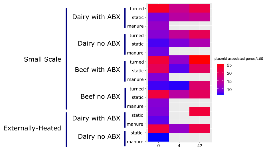
Fig. 4 Relative abundance of plasmid-associated genes annotated using the ACLAME database. Within the beef and dairy small-scale experiments, numbers increased significantly with time ( p = 0.03 , p = 0.02 ). Values plotted are averages, with n varying from 1 to 3 (see Fig. 2)
