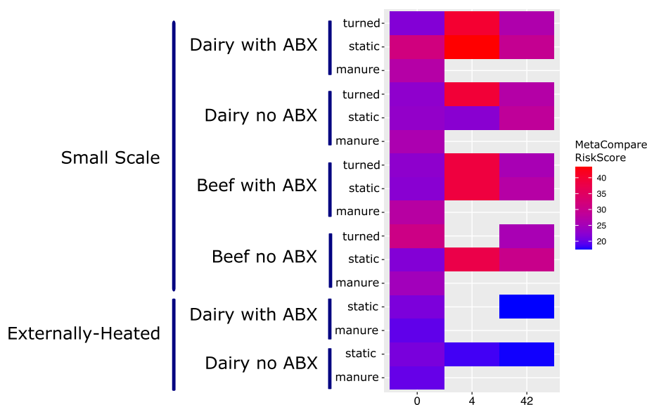
Fig. 5 Heatmap of MetaCompare resistome risk scores determined from all available metagenomics data sets. Factors that changed significantly with duration of composting: small-scale: all conditions/samples combined ( p = 0.0007 ), dairy conditions/samples combined ( p = 0.02 ), dairy turned condition ( p = 0.03 ). Externally heated: Both dairy with and without antibiotics decreased ( p = 0.04 , p = 0.04 ). Values plotted are averages of n varying from 1 to 3 (see Fig. 2)
