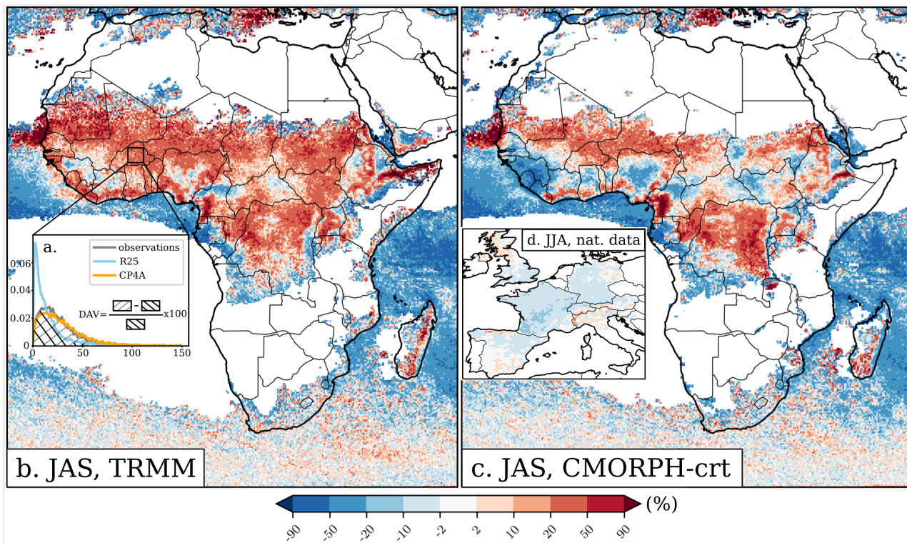
FIG. 1. Distribution added value (DAV) as defined by Soares and Cardoso (2018): a. (inset) Method: Fractional contribution of regular 1mmday -1 bins: the frequency in each bin is multiplied by its precipitation rate, and then normalized by mean precipitation. The overlap between each model and the observations is taken, and the DAV is the difference of overlap between CP4-Africa and the observations on the one hand and R25 and the observations on the other hand, normalized by the latter; b. DAV at every single grid-point for July-September daily precipitation distribution in CP4-Africa and R25 compared to TRMM observations, c. Same as b. but compared to CMORPHv1-crt observations. d (inset). DAV calculated over Europe with a similar model set-up run at 2.2km and 25km resolutions against national datasets (Berthou et al. 2020). The DAV is positive (red) when the precipitation distribution of the CPM overlaps more with the observations than the convection-parameterized model.
