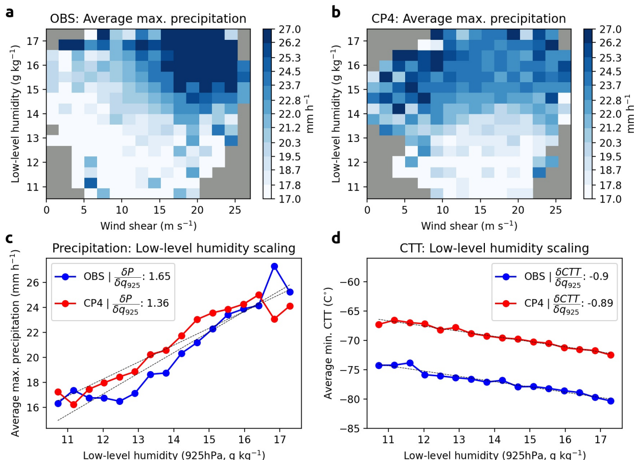
FIG. 2. MCS intensity scaling with atmospheric drivers for the CP4-Africa historical period and observations. 2d histograms for average maximum precipitation of (a) OBS and (b) CP4-Africa as a function of pre-storm (1200UTC) 925hPa specific humidity and 650-925hPa absolute zonal wind shear at storm location for > 24,000 afternoon (16-1900UTC) MCSs over the Sahel ( 12^{\circ}\text{W} - 12^{\circ}\text{E} ; 9 - 19^{\circ}\text{N} ). Bins with n < 10 MCSs are shaded grey. (c) depicts the average maximum precipitation for OBS (blue) and CP4-Africa (red) associated with humidity bins in (a,b). (d), as (c) but for minimum cloud top temperature (CTT). Legends show the slope of the linear fit (dashed lines). OBS combines ERA5 hourly data (wind shear and humidity), Meteosat Second Generation brightness temperatures (CTT, MCS defined as \geq 5000 \text{ km}^2 , \leq -50^{\circ}\text{C} ) and IMERG High Quality precipitation estimates (1mm minimum rainfall threshold) for 2004-2017.
