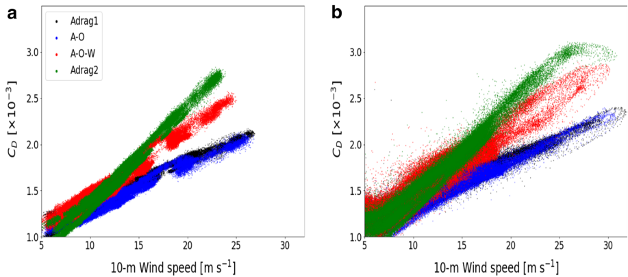
Fig. 10 Drag coefficient dependence on 10-m wind speeds computed as the value of C_D = \tau / \rho U_{10}^2 over a 15 \times 15 grid-cell area centred on points in the a North Sea ( 58.2^\circ N, 0.9^\circ E) for the Adrag1 (black), A–O (blue), A–O–W (red), and Adrag2 (green) parametrizations, and b North Atlantic Ocean ( 52.98^\circ N, 12.46^\circ W) configurations. Scatter points at hourly intervals from 0000 UTC 17 September to 0000 UTC 20 September 2018
