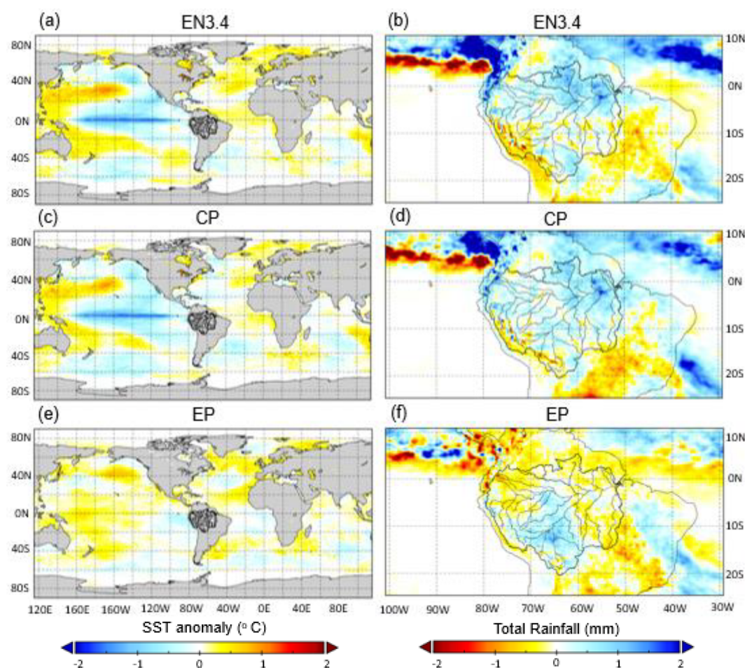
Figure 12. Composite analysis of the difference between the preceding OND average SST ( ^{\circ}\text{C} ) (a, c, e) and total rainfall (mm) (b, d, f) for the average of the 12 negative years and the average of the 12 neutral years. Panels (a, b): EN3.4 index; panels (c, d): CP index; and panels (e, f): EP index. A list of the negative and neutral years for each index can be found in Tables S2, S4 and S5 in the Supplement.
